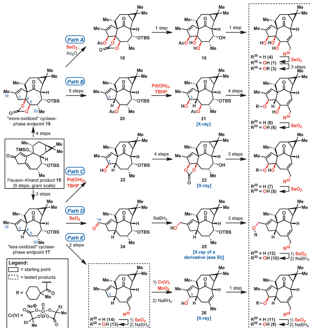
Figure 2. Overview of the synthetic sequence from Pauson–Khand product 15 to ingenol ( 1 ) and ingenol analogues 3–14 classified by oxidation level. Oxidation events are shown in red; other transformations have been abbreviated for overall clarity (see the Supporting Information). Ingenol analogues used for biological testing are placed within dotted boxes.
