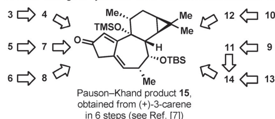
Figure 1. A) Previously synthesized ingenane targets: ingenol ( 1 ), ingenol mebutate ( 2 ; the active ingredient in Picato), and an ester derivative 3 . B) Current ingenane targets with varying oxidation states. C) A synthetic plan that maximizes divergency from previously synthesized intermediate 15 .
